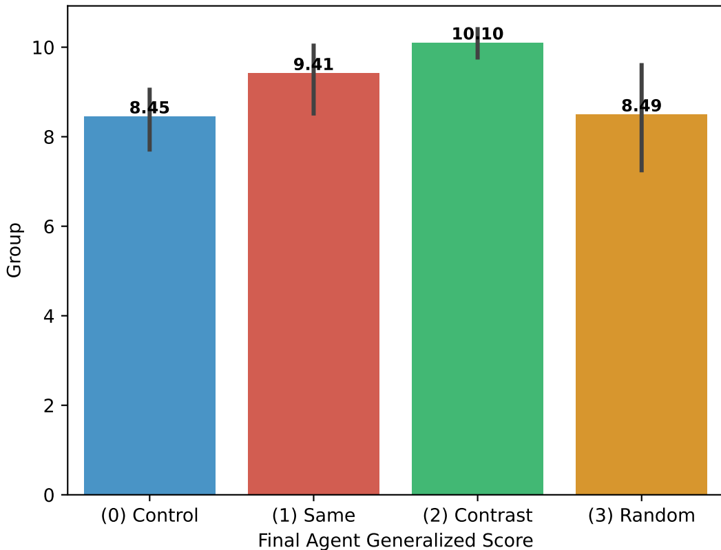
Final Agent Generalized Score by Group
